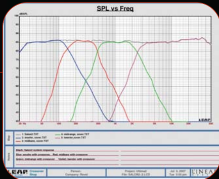
Response curves indicating the exemplary acoustic output of each filter network section with its associated transducers in a Salon2 loudspeaker
